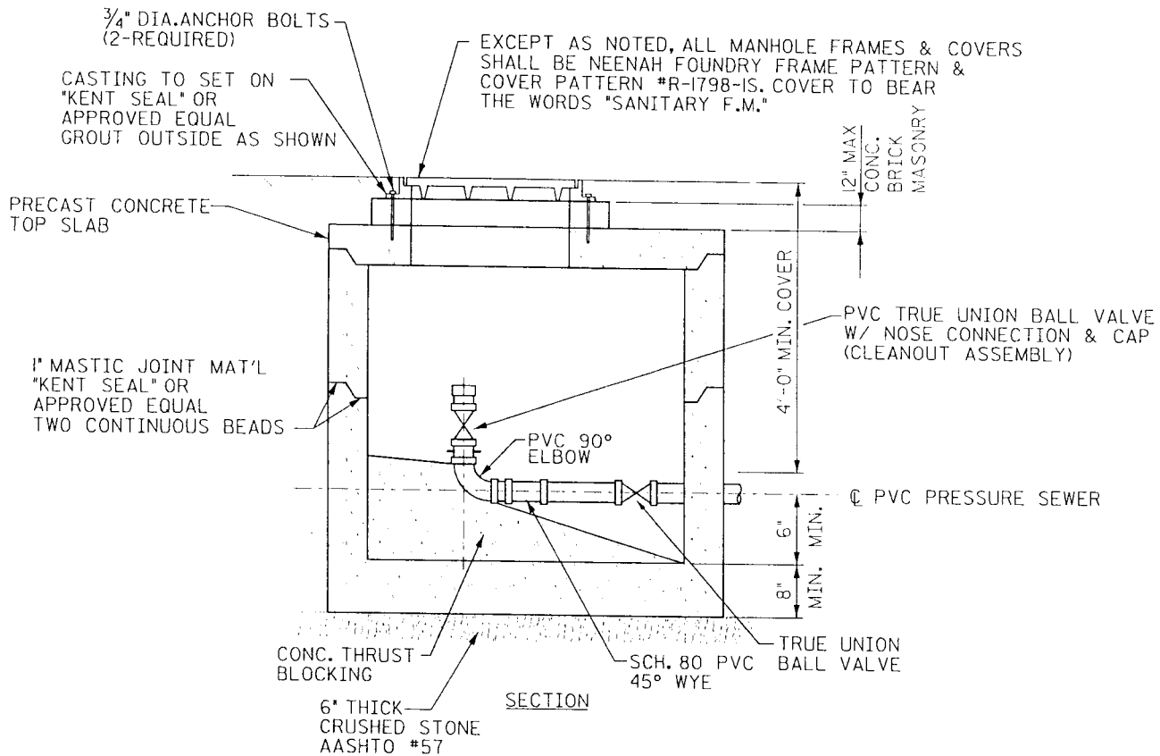
PRESSURE SEWER SERVICE LINE CONNECTION W/ TERMINAL CLEANOUT NOT TO SCALE
