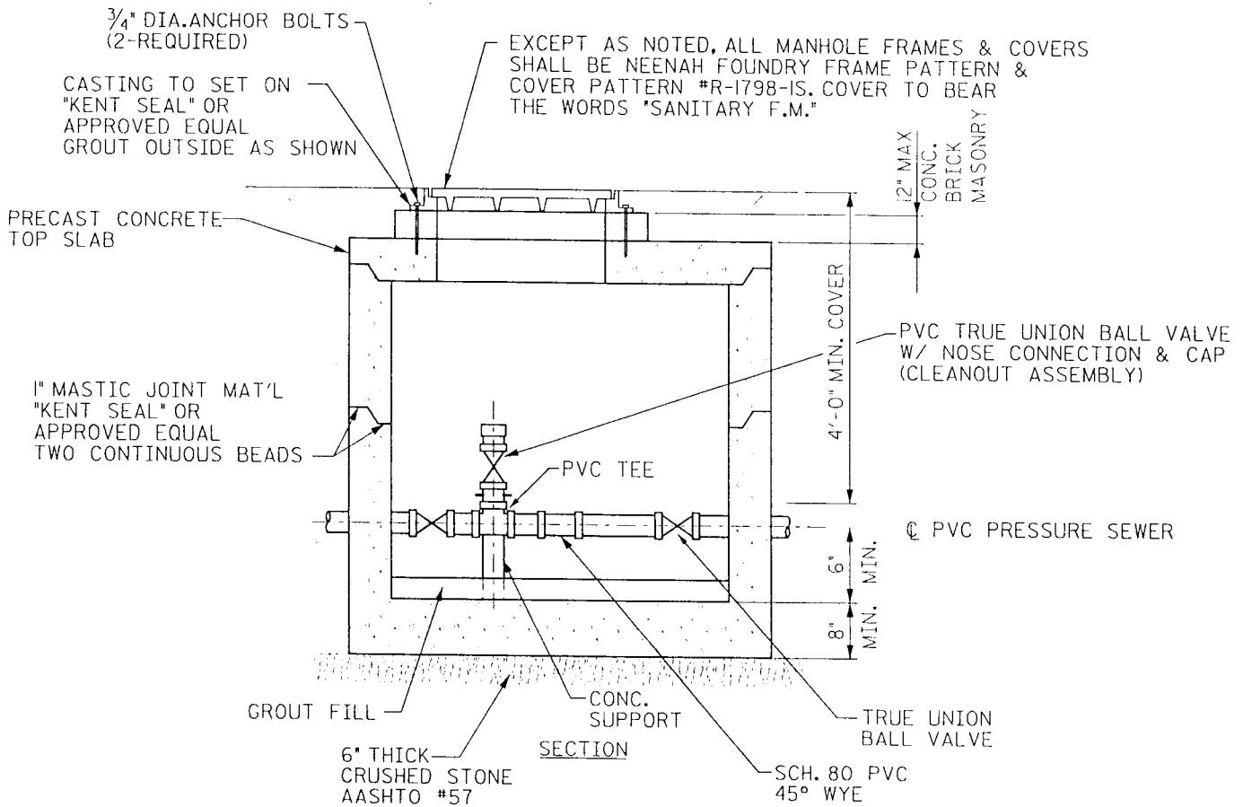
PRESSURE SEWER SERVICE LINE CONNECTION W/ INLINE CLEANOUT NOT TO SCALE
