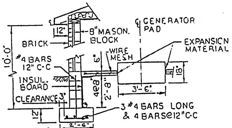
TYPICAL WALL DETAIL
